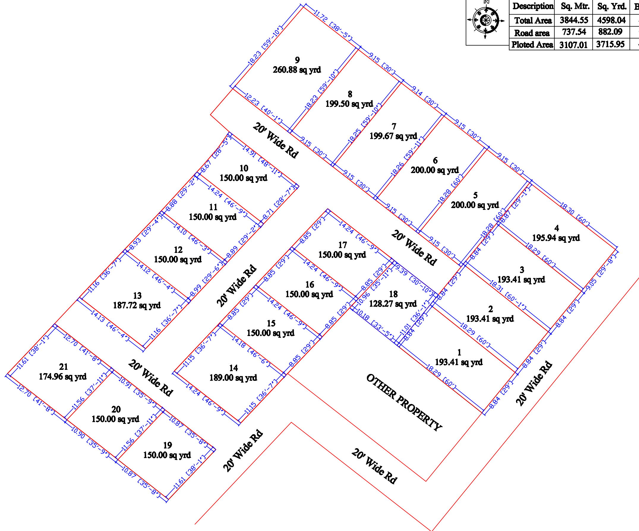
LAYOUT PLAN AT SHERPUR
